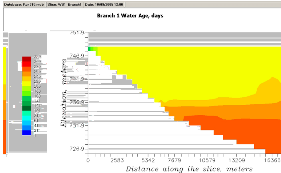
Figure 6-13 Water age during a period of low inflow and stratification
