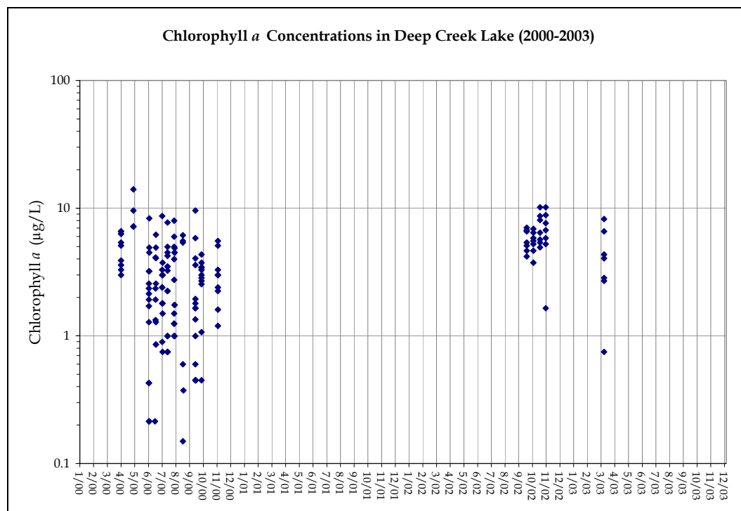
Figure 4-1 Deep Creek Lake chlorophyll a concentrations (source: MDE)
